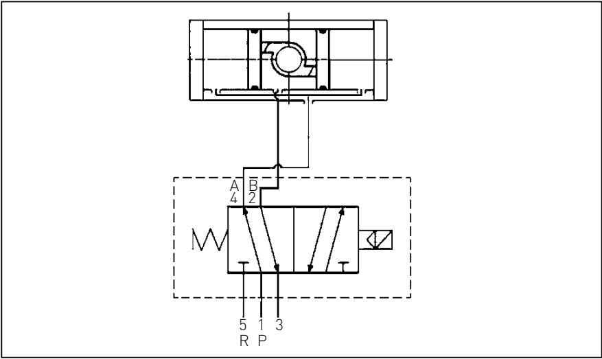
Double acting with Namur 5/2 way valve
