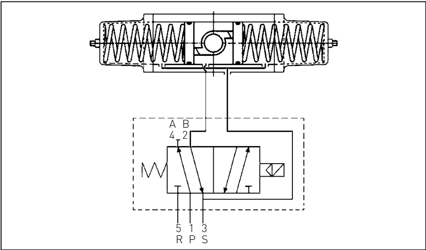
Single acting with Namur 5/2 way valve
