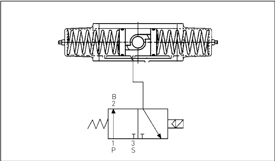
Single acting with 3/2 way valve
